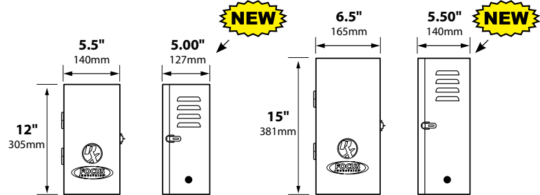
Mechanical Timer (-T) & Remote Photo Cell (-RXTRPC)
