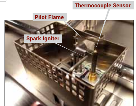
PILOT ASSEMBLY AND BLOWOUT BOX
