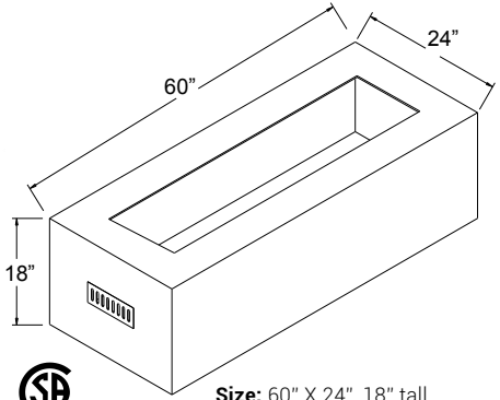
Size: 60" X 24", 18" tall Insert: 30" X 12" or 36" X 14"
